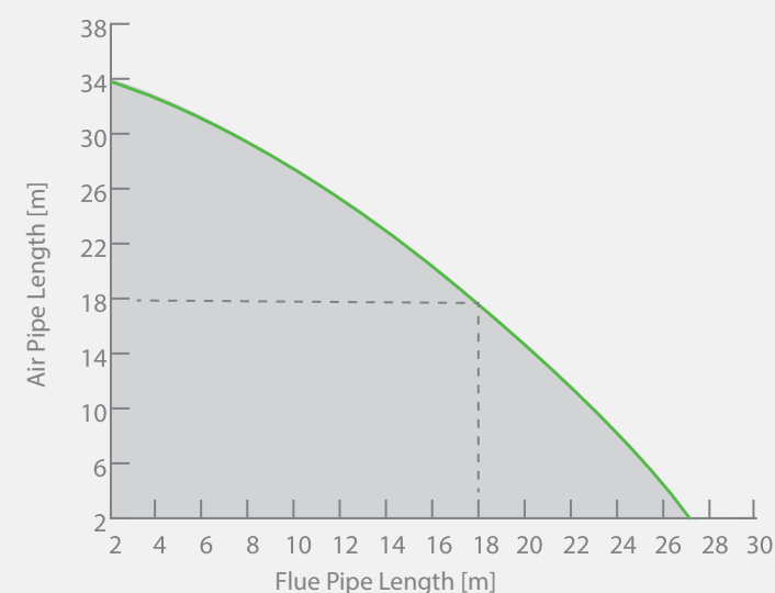
Keston Combi C30 - Flue & Air Pipe Length
